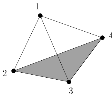
Figure 3: The Nim-regular complex of Example 4.6.
