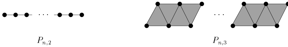
Figure 5: The path complexes P_{n,2} and P_{n,3} .
